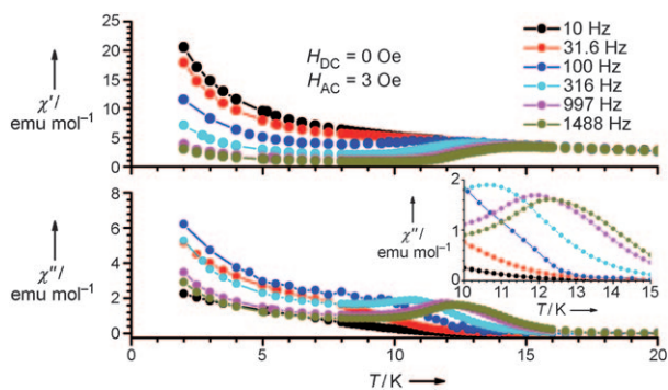
Figure 2. The temperature dependence of ac susceptibility at frequencies from 10 to 1488 Hz for the undiluted \text{Dy}^{3+} complex.
